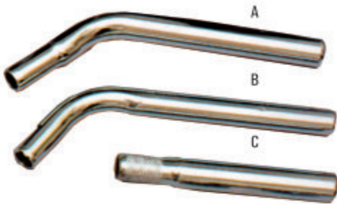
GS-82 : Made of quality (ERW) steel tube ZP/BNCP finish A) for BMX Diam :22.2mm (7/8") Length 250mm & 280mm B) for BMX Diam : 25.4mmx22.2mm(7/8") Length 325-380mm C) for roadster bicycles Diam : 25.4mm(1")x 22.2mm (7/8") length to order
